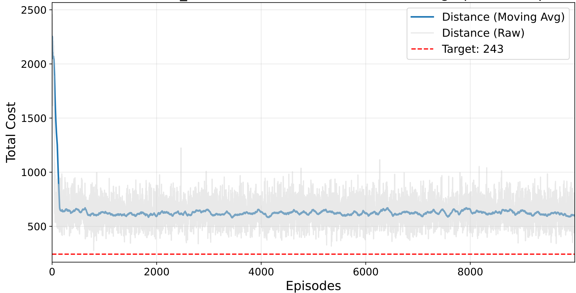
Final RANDOM_SEARCH Masked AutoRL-SOP Training - prob.42.sop
